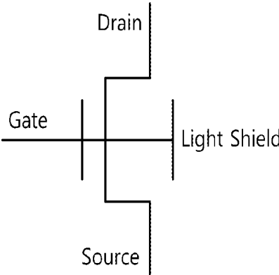
< Double gate >
