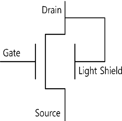
< Drain-LS contact >
